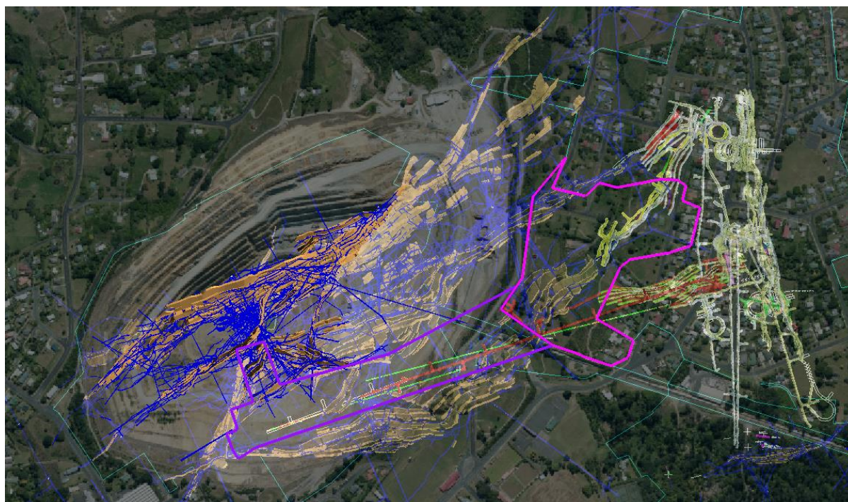
Figure 1. General overview of the Martha Underground Mine Area in relation to historical workings.
