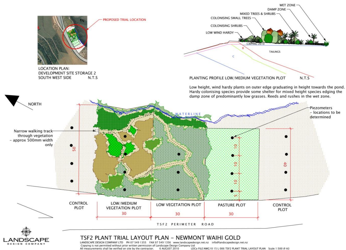
Figure 13 – Location and Trial Layout Plans for Tailings Revegetation Trial
