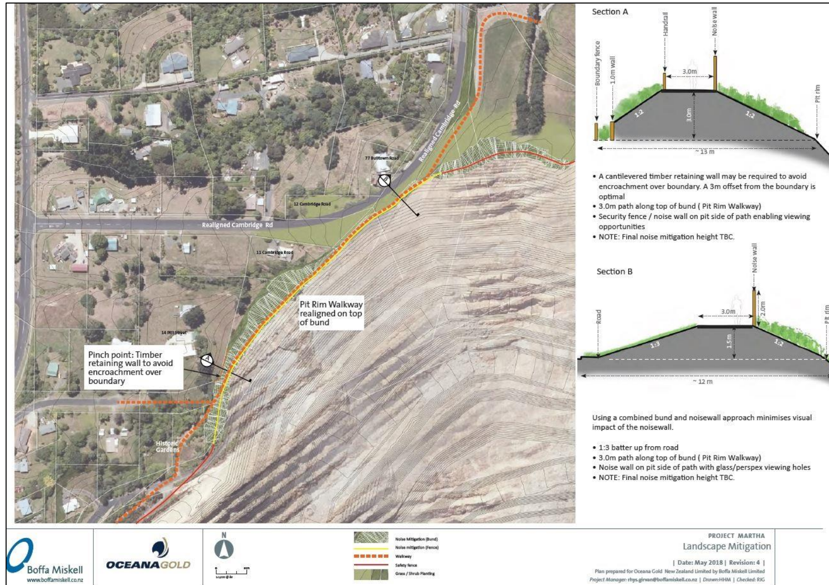
Figure 3: North Wall Realignment
