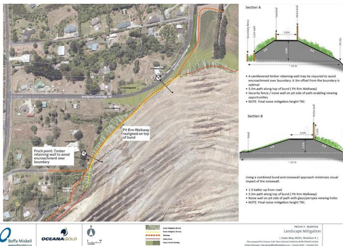
Figure 7: Project Martha Pit Rim Walkway Realignment
