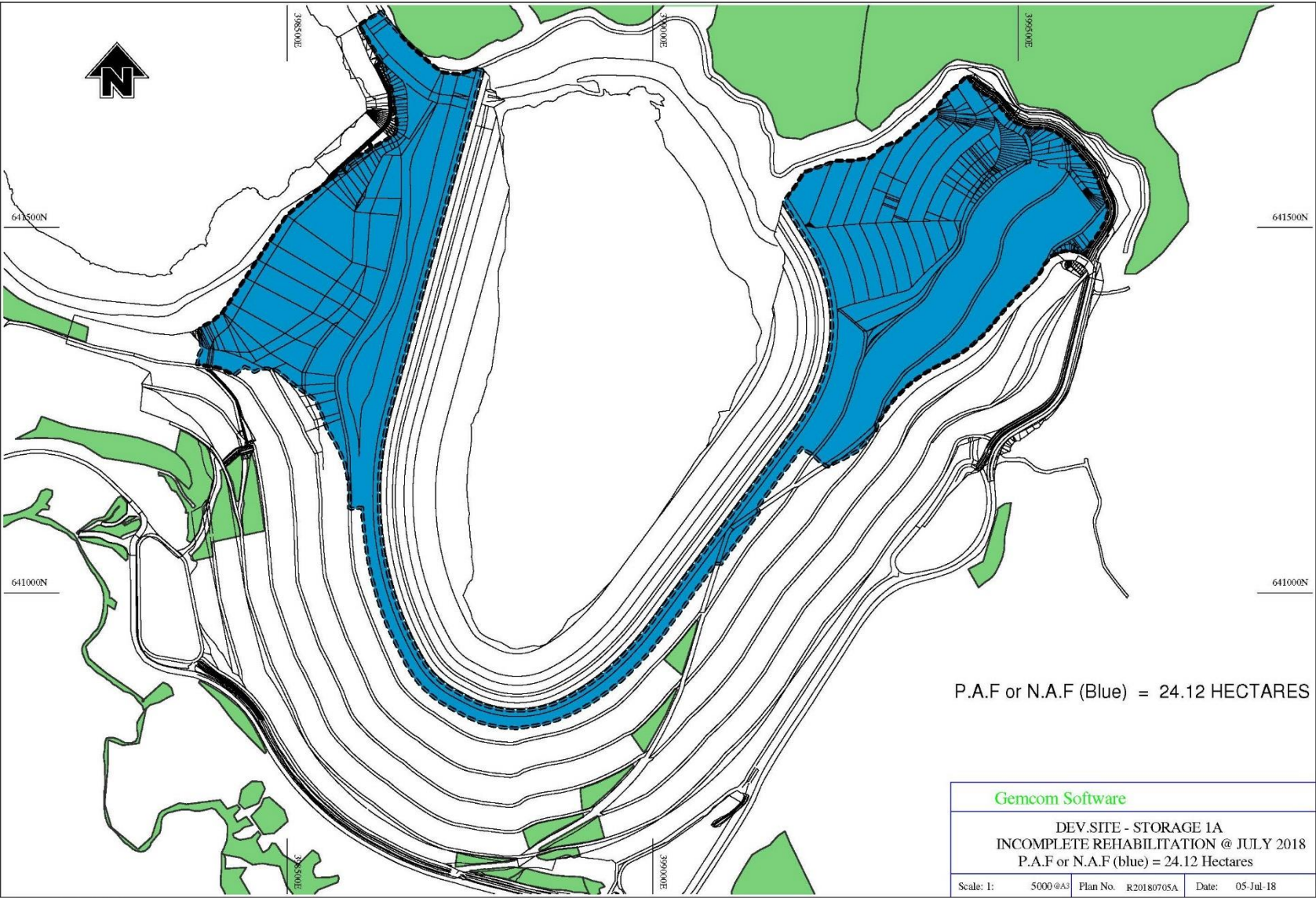
Figure 5: TFS1A Areas for Rehabilitation
